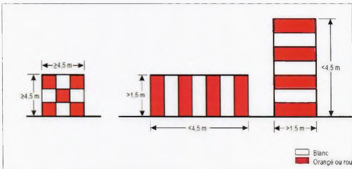
Figure 6-1. Marquages types
